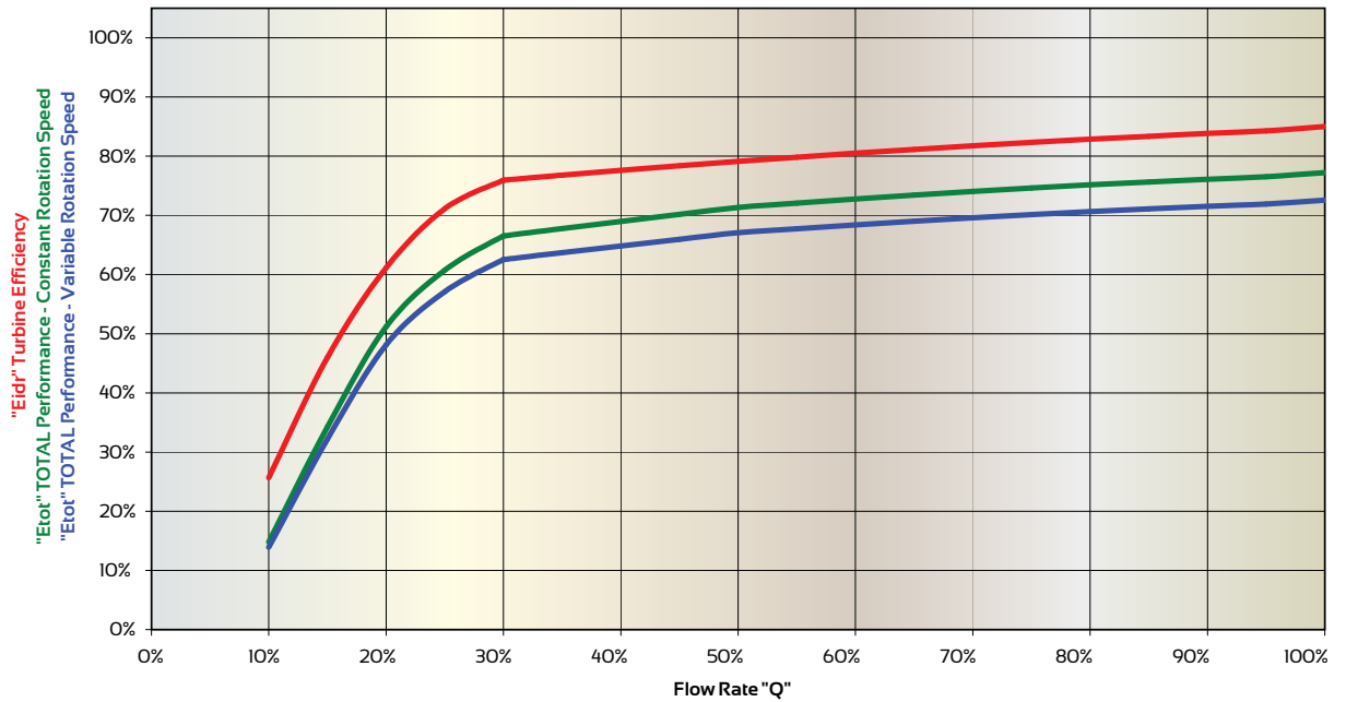
Water Flow Rate / Efficiency PAE Hydrodynamic Screw with "Constant Rotation Speed" or "Variable Rotation Speed"
